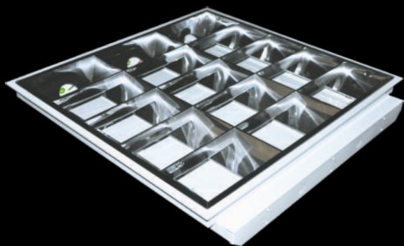
F57/3X10W/LED L595XW595XD75MM Recessed Empty Body
