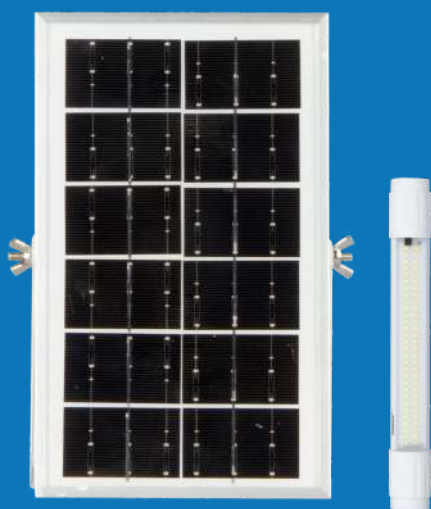
ES169/LED/SL/80W (8874) SOLAR LED TUBE LIGHT 80W, Ø34XL850MM, IP54, ABS With Polycrystalline silicon Solar Panel, Remote, Li-ion Batteries and a 5m Cable Charging time: 6-8H, Working time: 8-10H
